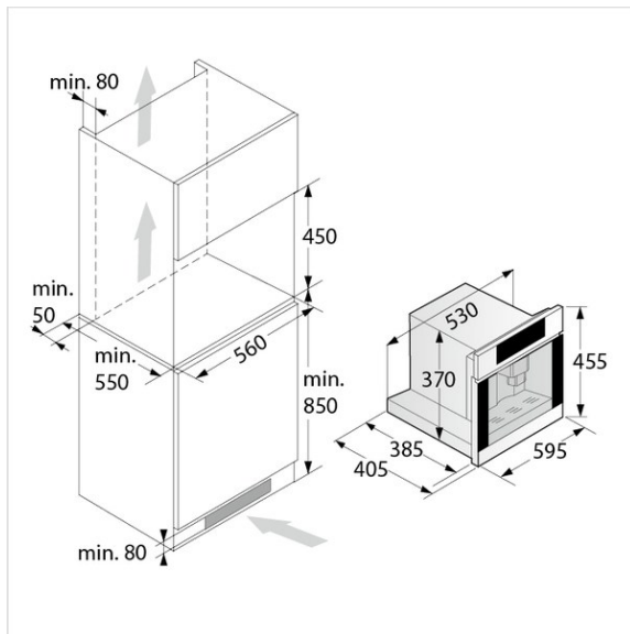
CM8457S Skizze
