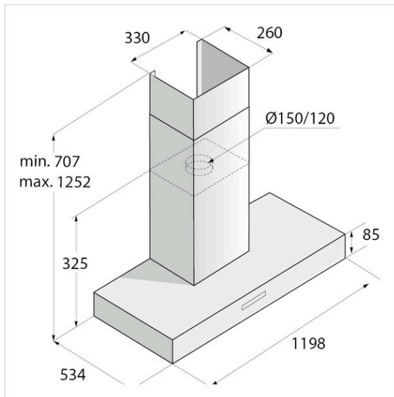
CW41230G Skizze
