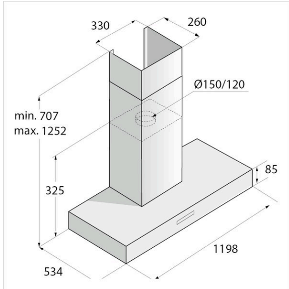
CW41230G Skizze
