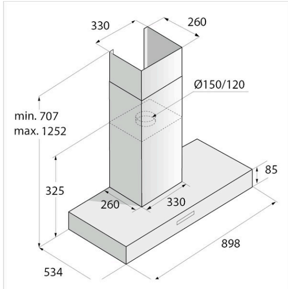
CW4930G Skizze
