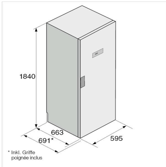
DC7784HPW Skizze
