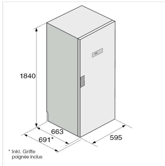
DC7784HPW Skizze
