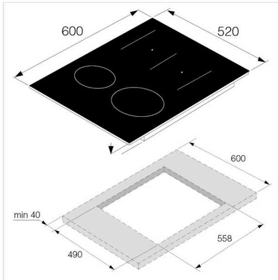
HI1621G Skizze
