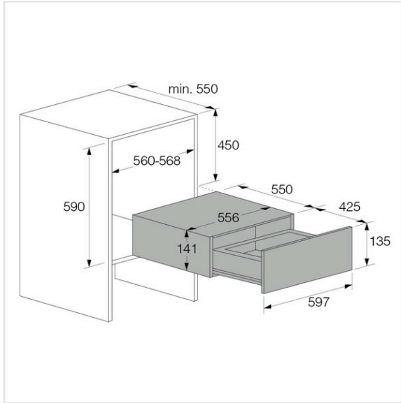
ODV8127B Skizze
